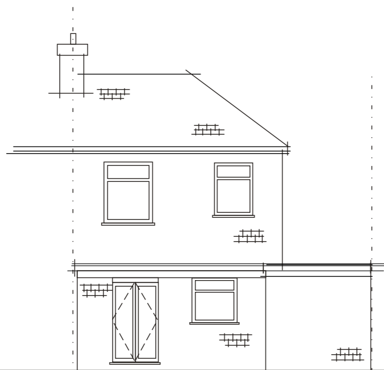
EXISTING REAR ELEVATION (SOUTH)
